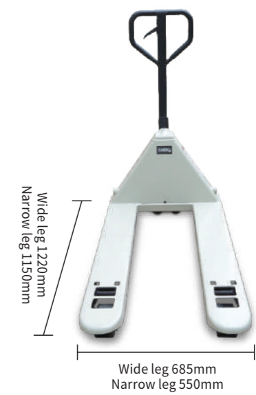
If the distance between pallet positions is greater than 700mm , choose Wide leg 685 specification
